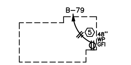
METALIZER PIT RECEPTACLE PLAN SCALE: 1/16" = 1'-0"
